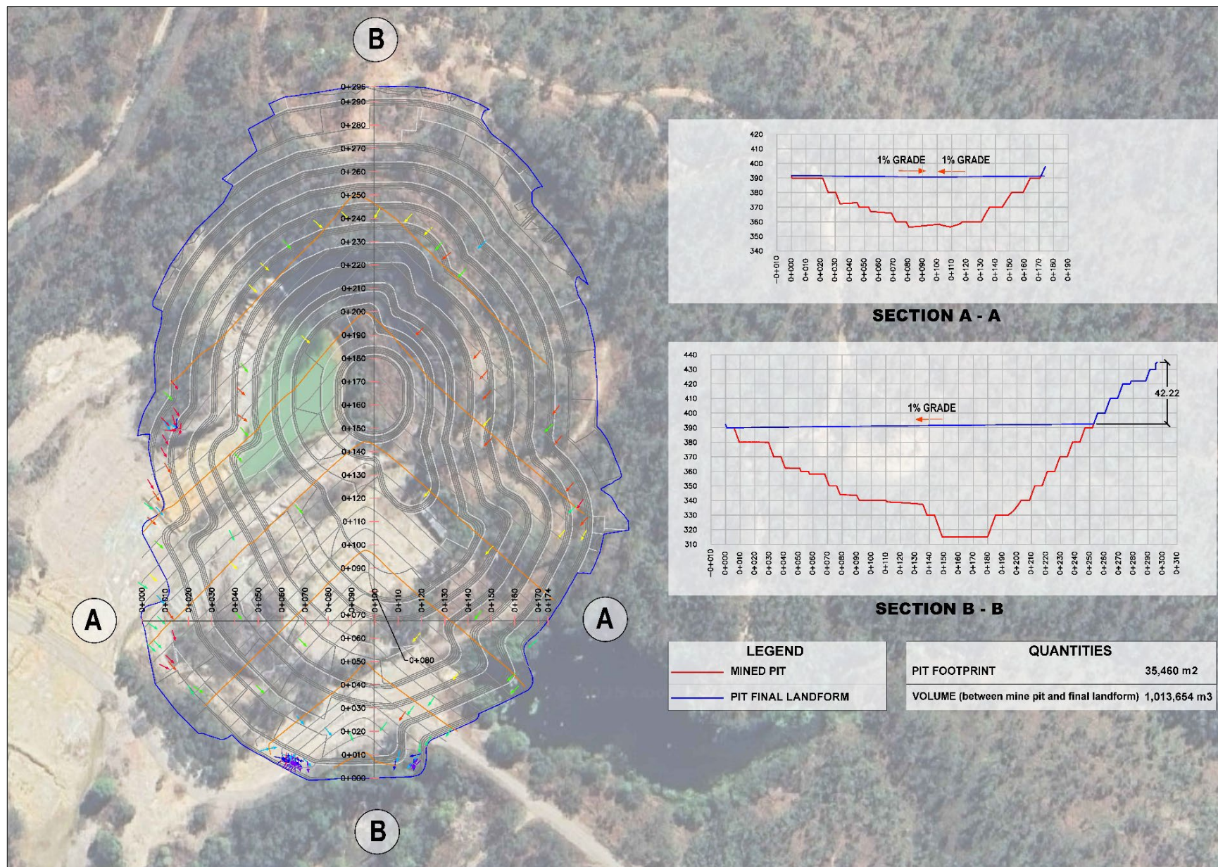
Appendix 2.9 - Figure 8: Backfilled Pit
