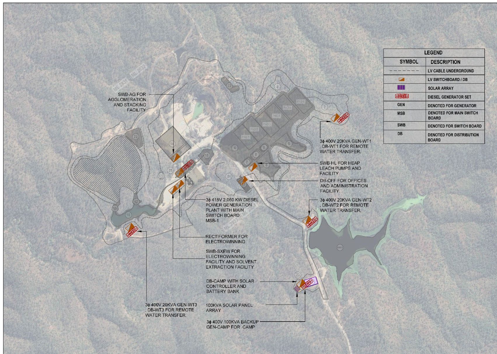
Appendix 2.4 - Figure 2c: Project Layout – Mine Electrical Reticulation
