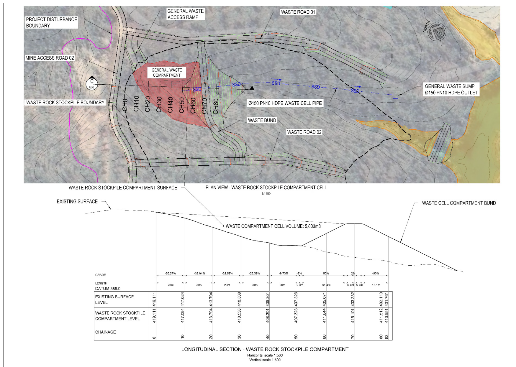
Appendix 2.11 - Figure 12a: Predicted Landfill Layout – Plan and Cross Section
