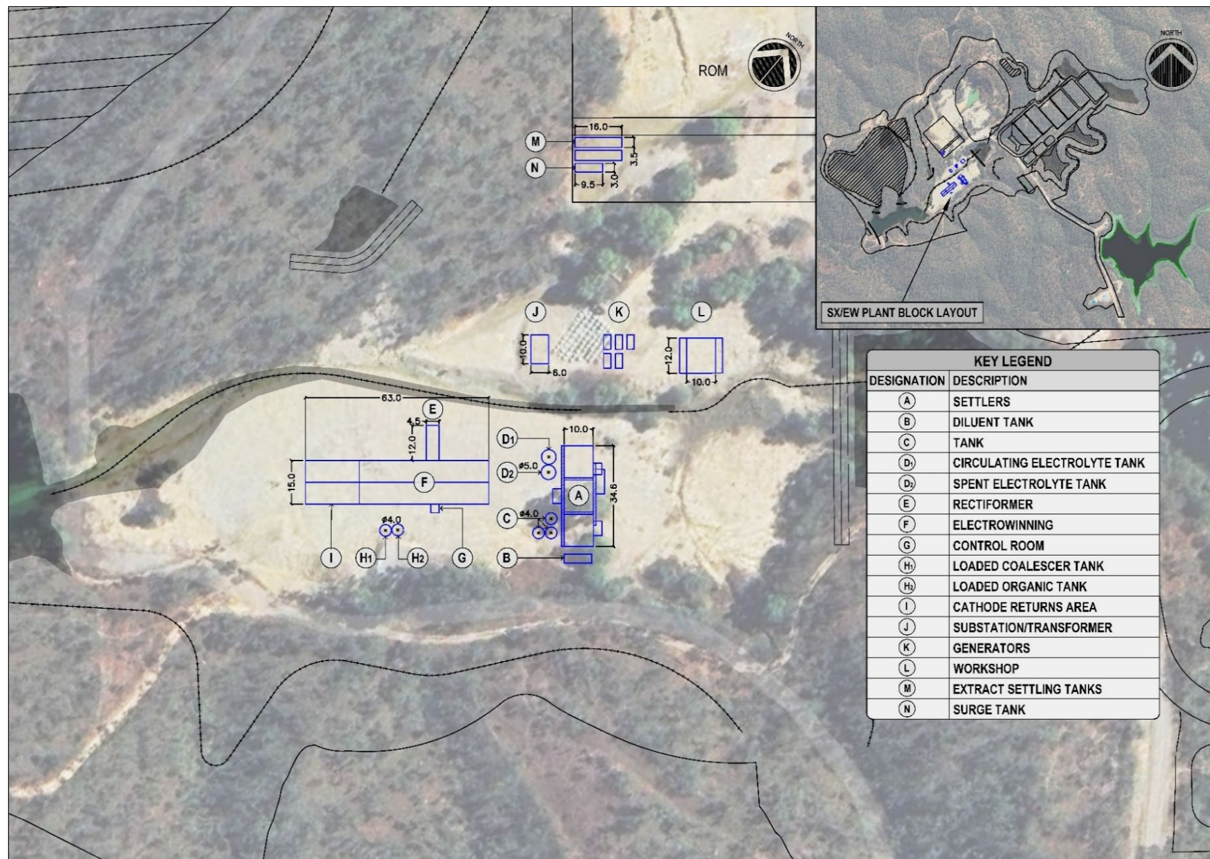
Appendix 2.6 - Figure 4: Indicative Processing Infrastructure Layout
