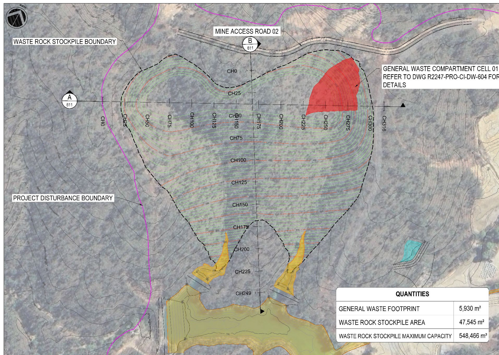
Appendix 2.10 - Figure 12: Predicted Landfill Layout
