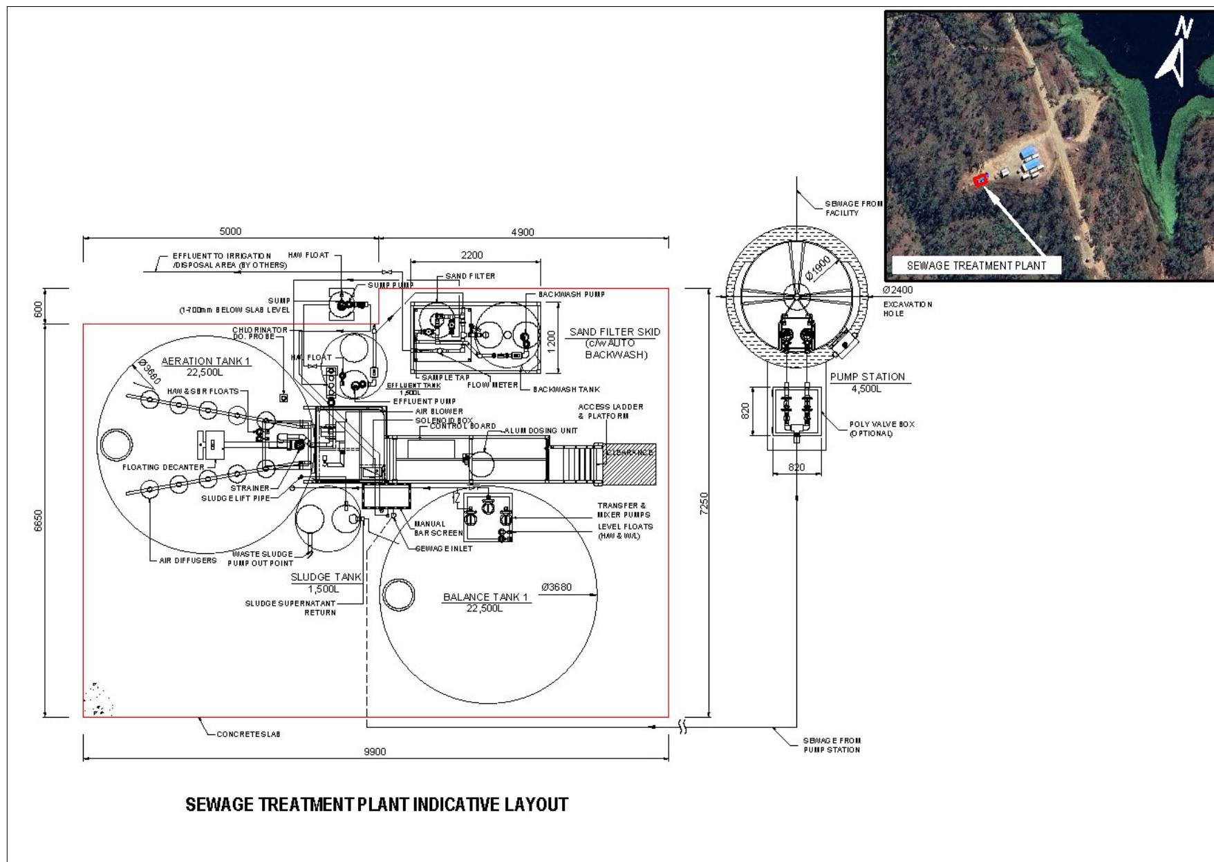
Appendix 2.2 - Figure 2a: Project Layout – Sewage Treatment Plant Location
