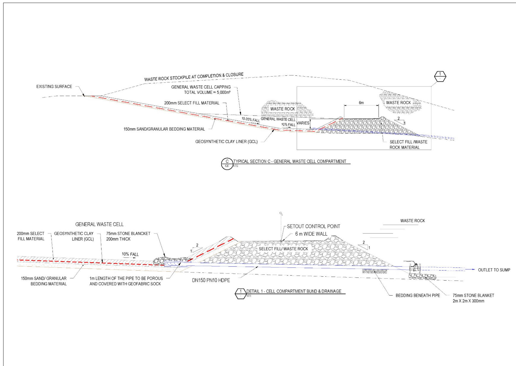
Appendix 2.12 - Figure 12b: Predicted Landfill Layout – Detailed Cross Section
