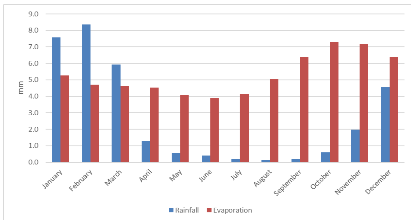
FIGURE 3.1: AVERAGE DAILY RAINFALL AND EVAPORATION
