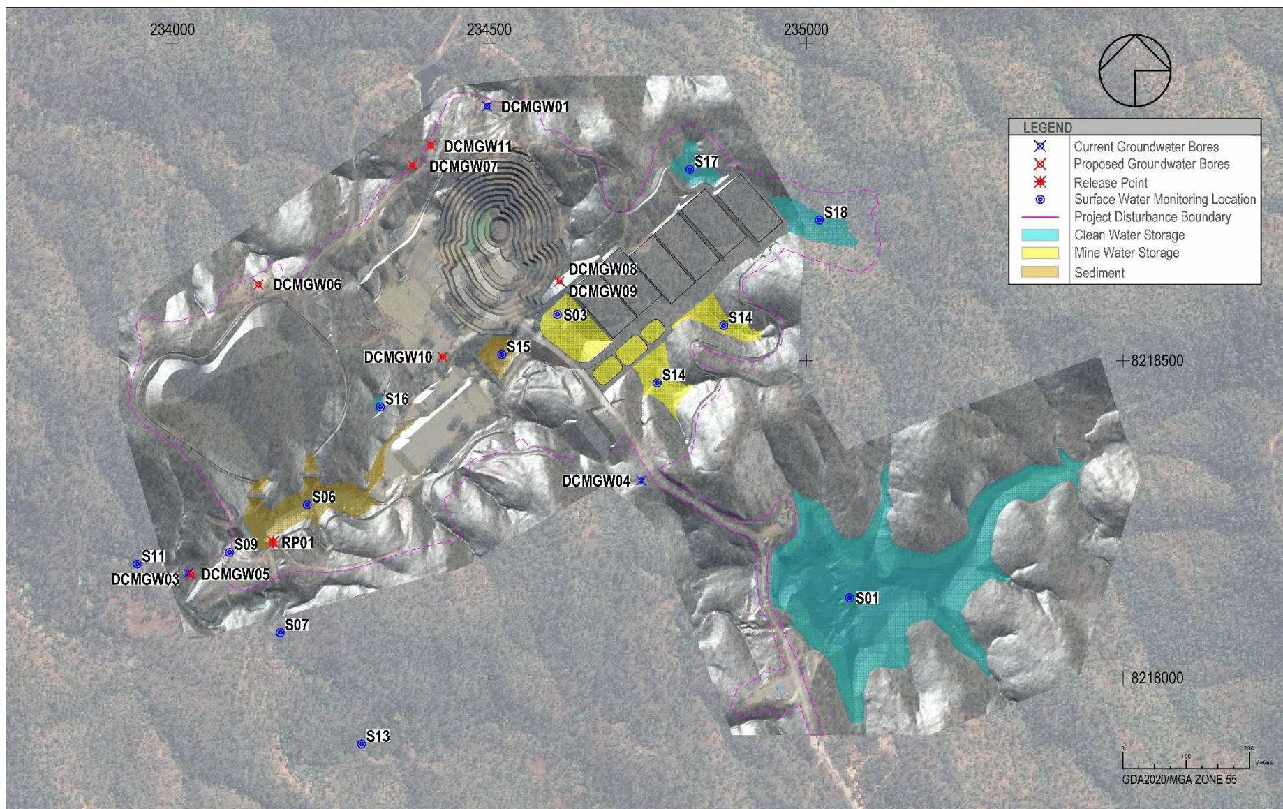
FIGURE 8.1: OPERATIONAL WATER MONITORING LOCATIONS
