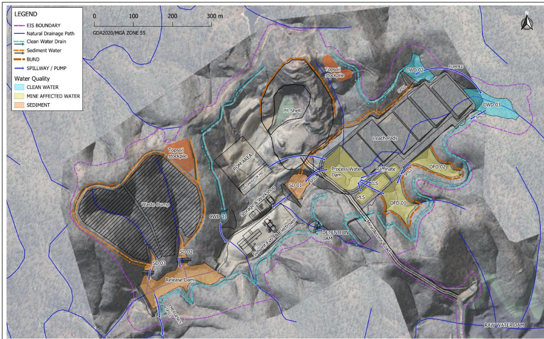
FIGURE 4.3: PROPOSED WMS PLAN
