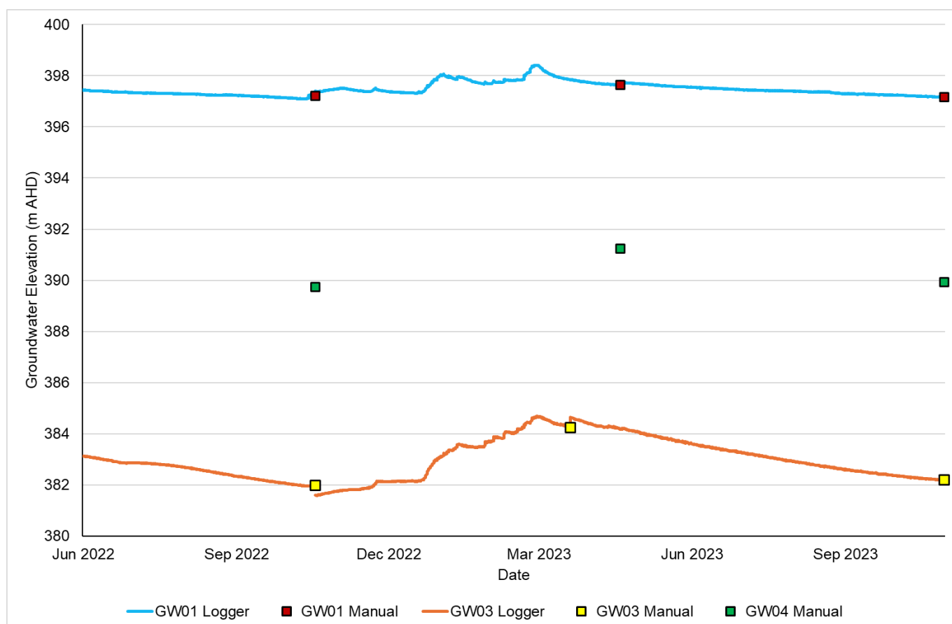
FIGURE 3.4: GROUNDWATER LEVELS
